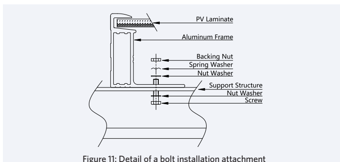
Figure 11: Detail of a bolt installation attachment
